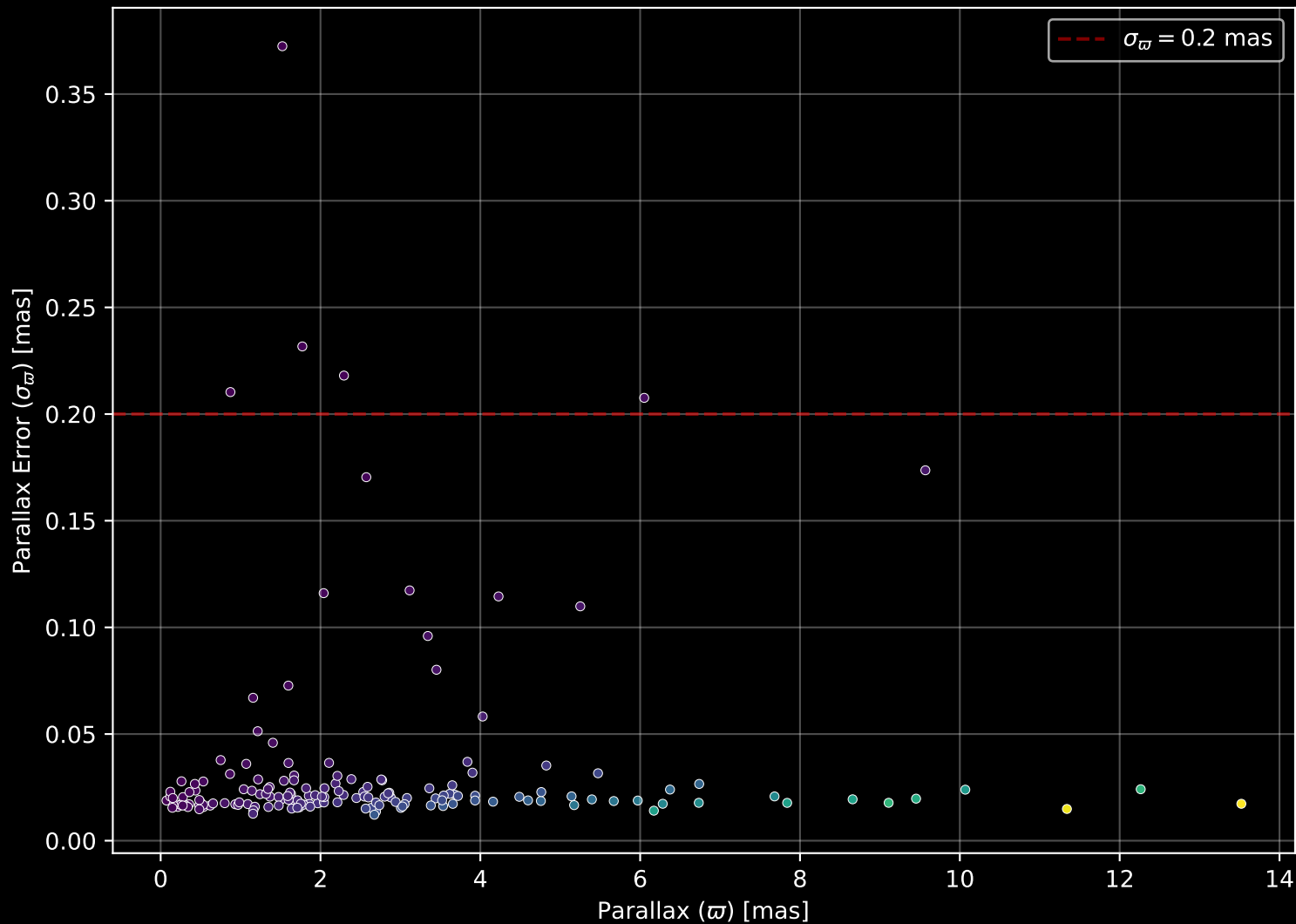
APOGEE DR17 Field: [047-40_MGA] Parallax Quality (n= 168)
