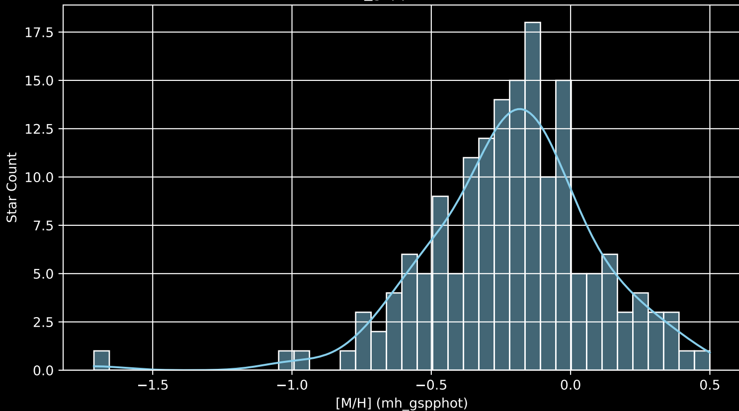
APOGEE DR17 Field: [047-40_MGA [M/H] (mh_gspphot) (n= 164)
