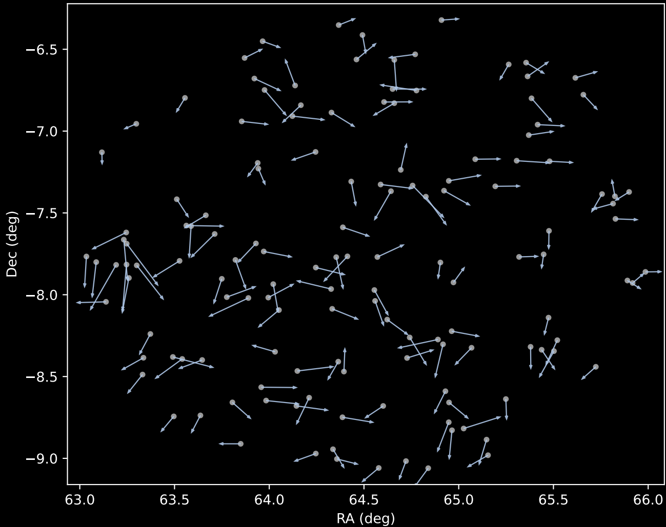
APOGEE DR17 Cluster 1 Proper Motion Vectors (n=139)
