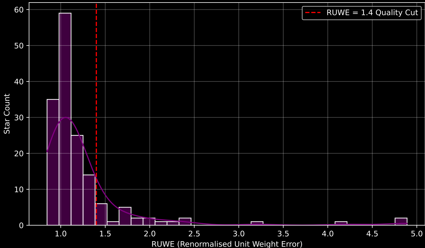
GAPOGEE DR17 Field [047-40_MGA] RUWE Distribution (n= 157)
