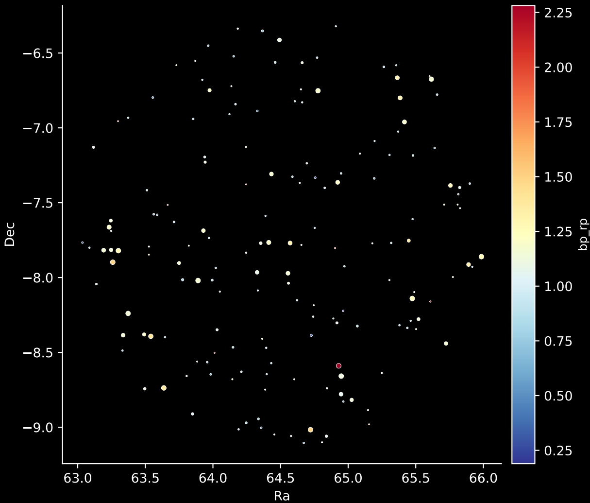
APOGEE DR17 Field: [047-40_MGA] Stars: 168
