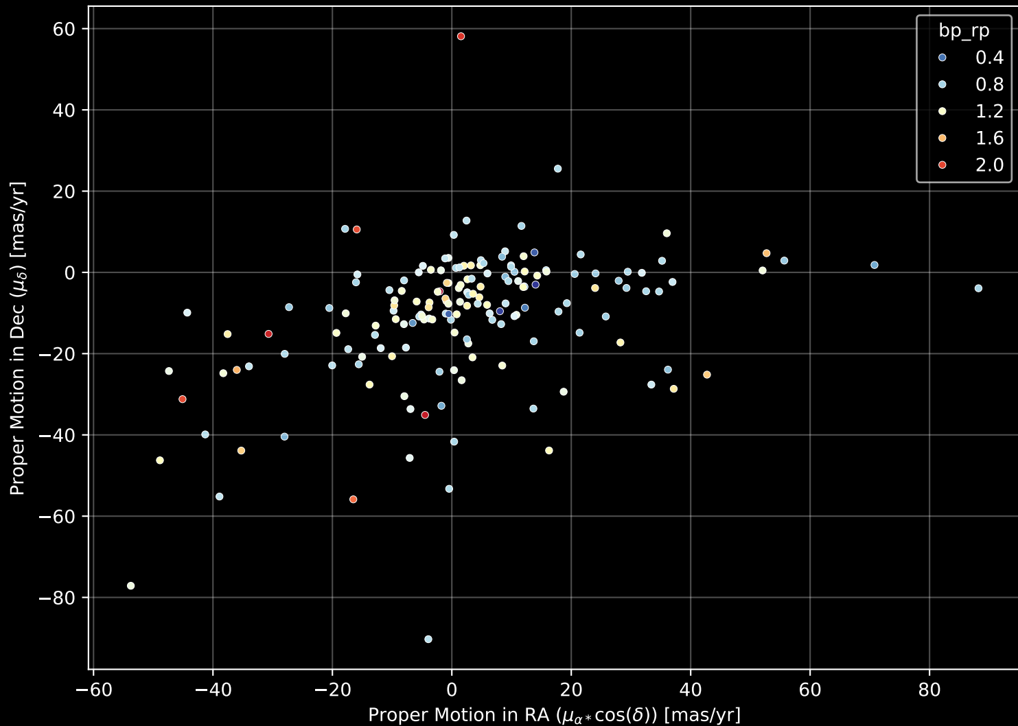
APOGEE DR17 Field: [047-40_MGA] Proper Motion Diagram (n= 168)
