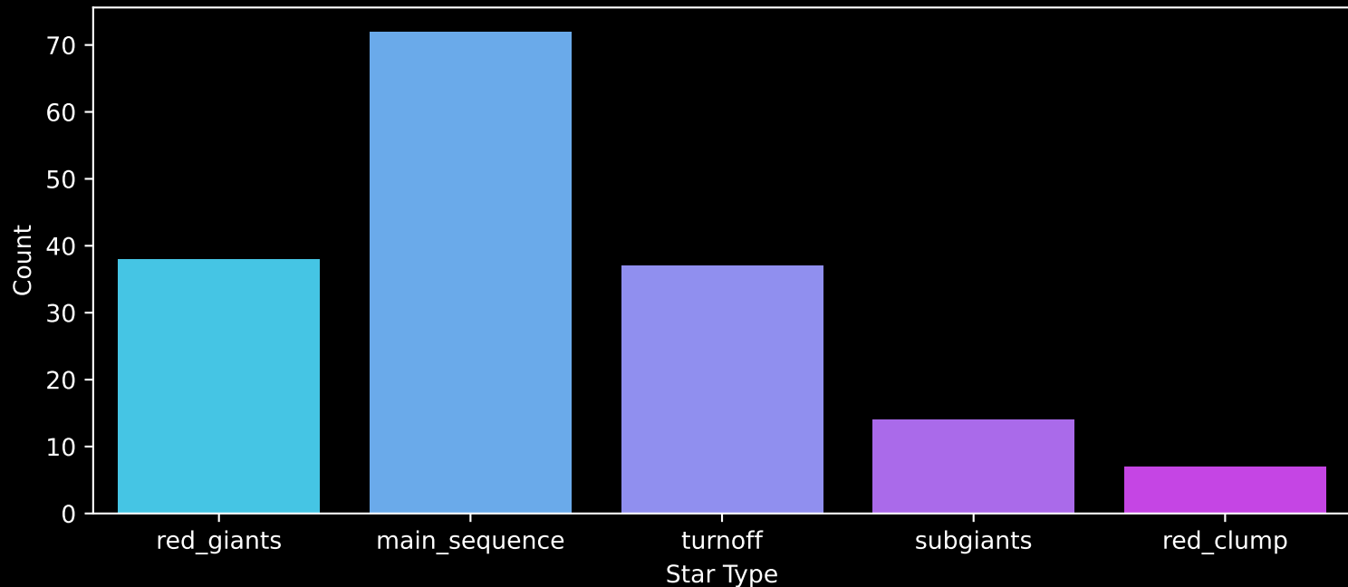
APOGEE DR17 Field: [047-40_MGA] Count plot of Star Type
