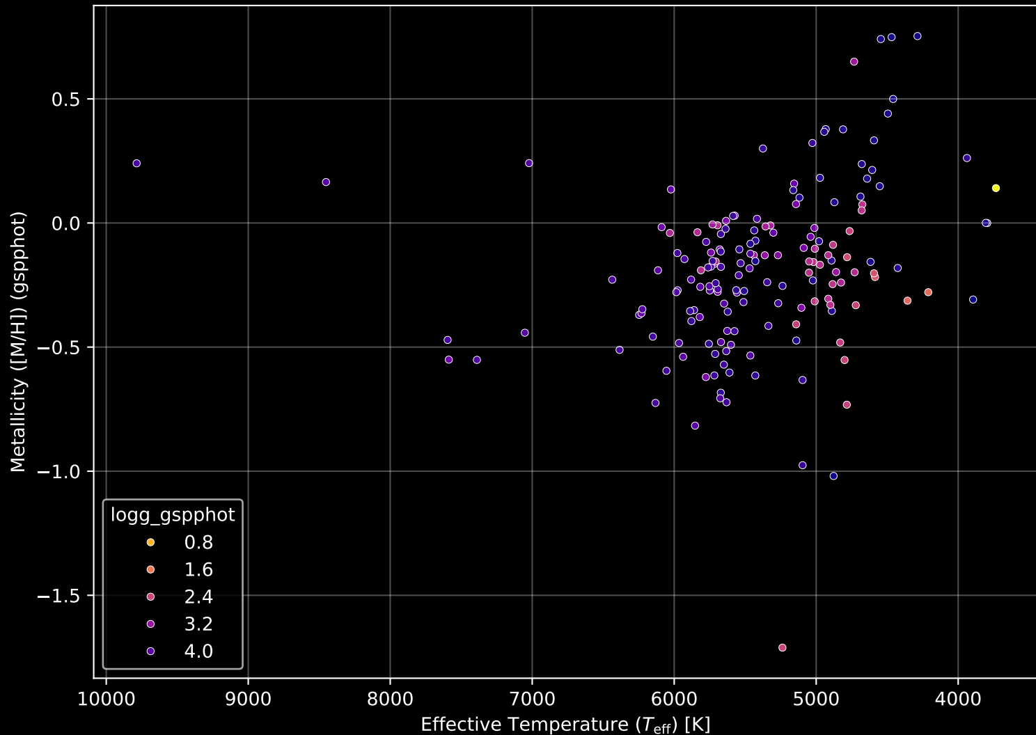
APOGEE DR17 Field: [047-40_MGA] Stellar Population Parameters (n= 168)
